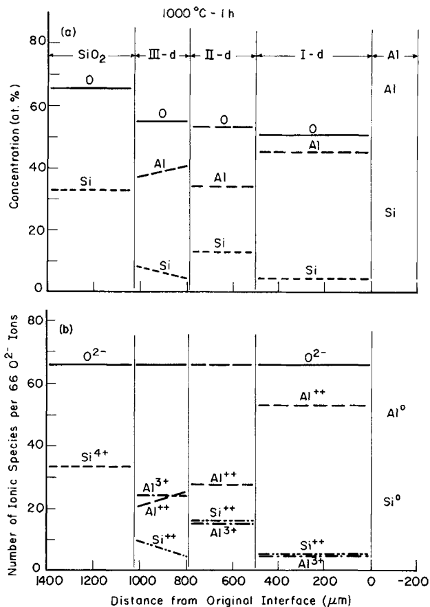
Figure 6 (a) Electron microprobe analysis in at. % of a cross-section of an Al-SiO 2 specimen after reacting at 1000° C for 1 h. (b) Calculated ionic species profiles based on a constant number of oxygen ions using at. % concentration data in (a).
