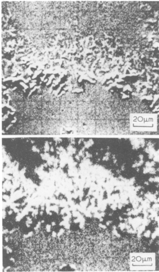
Figure 8 X-ray fluorescence micrographs of the cross-section of a specimen after reacting at 900° C for 1 h showing layers I-a (top), II-a, and III-a: (top) AlK \alpha , (bottom) SiK \alpha .
