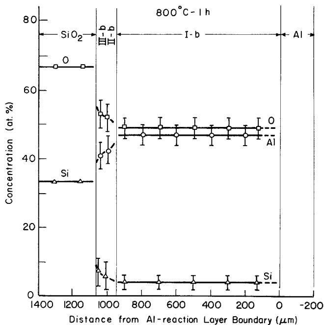
Figure 5 Electron microprobe analysis in at. % of a cross-section of an Al– \text{SiO}_2 specimen after reacting at 800^\circ\text{C} for 1 h.
