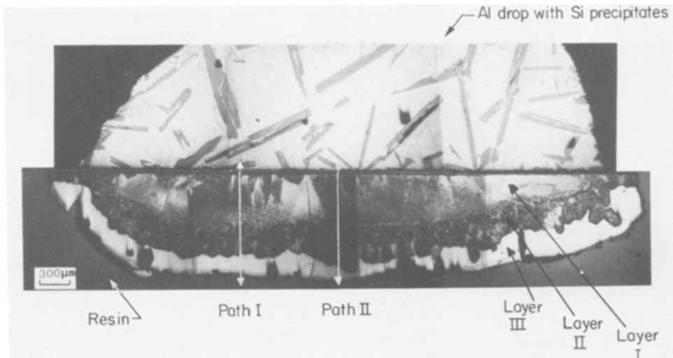
Figure 4 Optical micrograph of cross-section of an Al-fused \text{SiO}_2 specimen after reacting at 1000^\circ\text{C} for 1 h.
