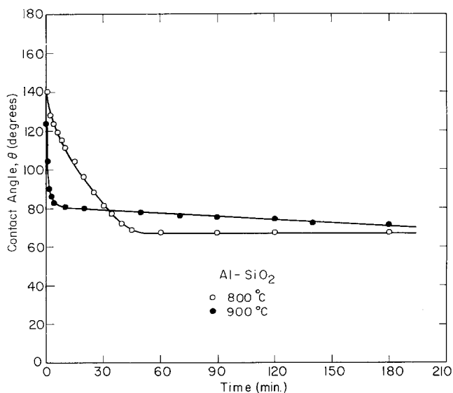
Figure 2 Change in advancing contact angle with time at 800 and 900° C.
