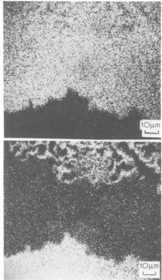
Figure 9 X-ray fluorescence micrographs of the cross-section of an Si-saturated Al (Al-28.3 wt.% Si)-SiO 2 specimen after reacting at 800° C for 24 h showing layers II-c (top), III-c, and SiO 2 : (top) AlK \alpha , (bottom) SiK \alpha .
