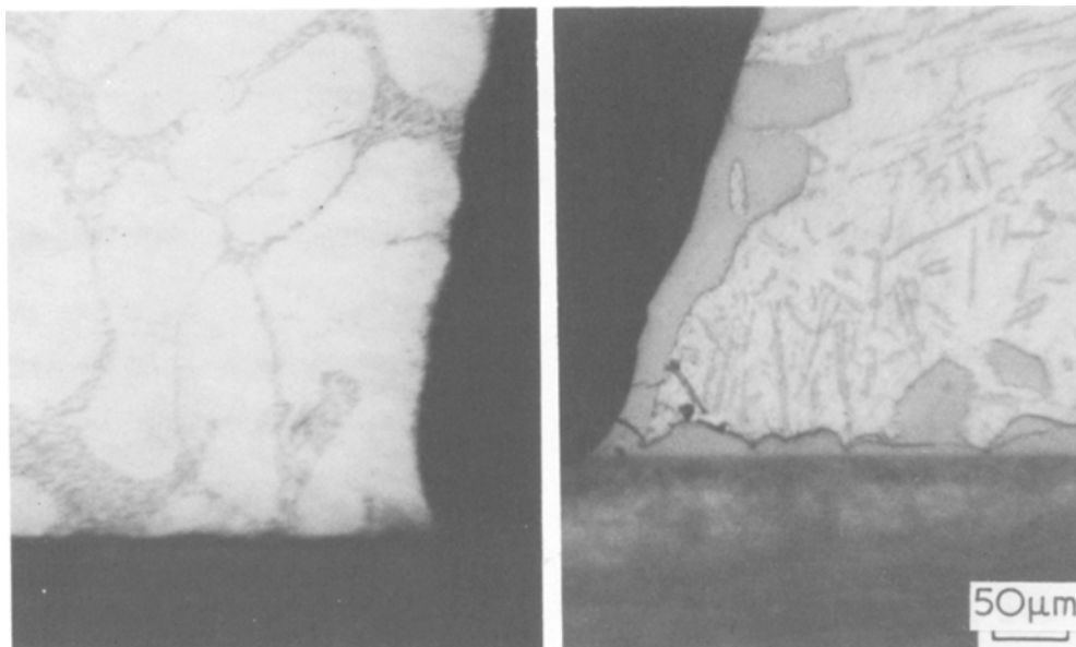
Figure 3 Optical micrographs of Al drop after reaction with SiO 2 at 800° C: (left) for 17 min, Al grains interspersed with Al-Si eutectic; (right) for 40 min, Si grains interspersed with Al-Si eutectic.
