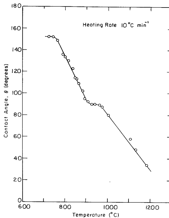
Figure 1 Change in advancing contact angle with temperature.
