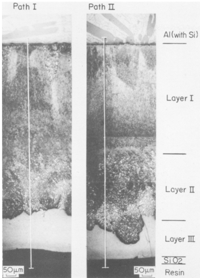
Figure 7 Enlargement of the areas along the two microprobe paths shown in Fig. 4 indicating layers I-d (top), II-d, III-d, and SiO 2 (bottom).
